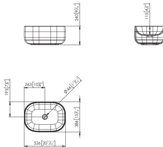
UNIQUE B812 52X38 1100 ON TOP
