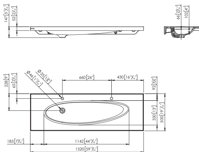
ENCIMERA NEST 152 CASSETTO DEL MOBILE NEST 152 PLAN VASQUE NEST 152
