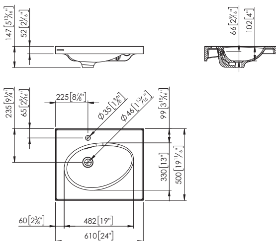
ENCIMERA NEST 61 CASSETTO DEL MOBILE NEST 61 PLAN VASQUE NEST 61
